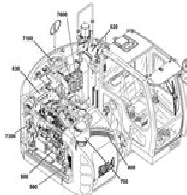
Fig. 1-4 Upper carriage
