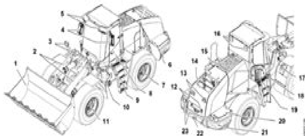
Fig. 1: Overview of the entire machine
