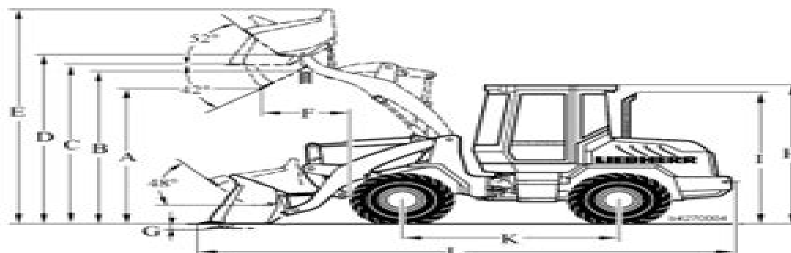
Dimensions – machine with Z-bar lift arms
