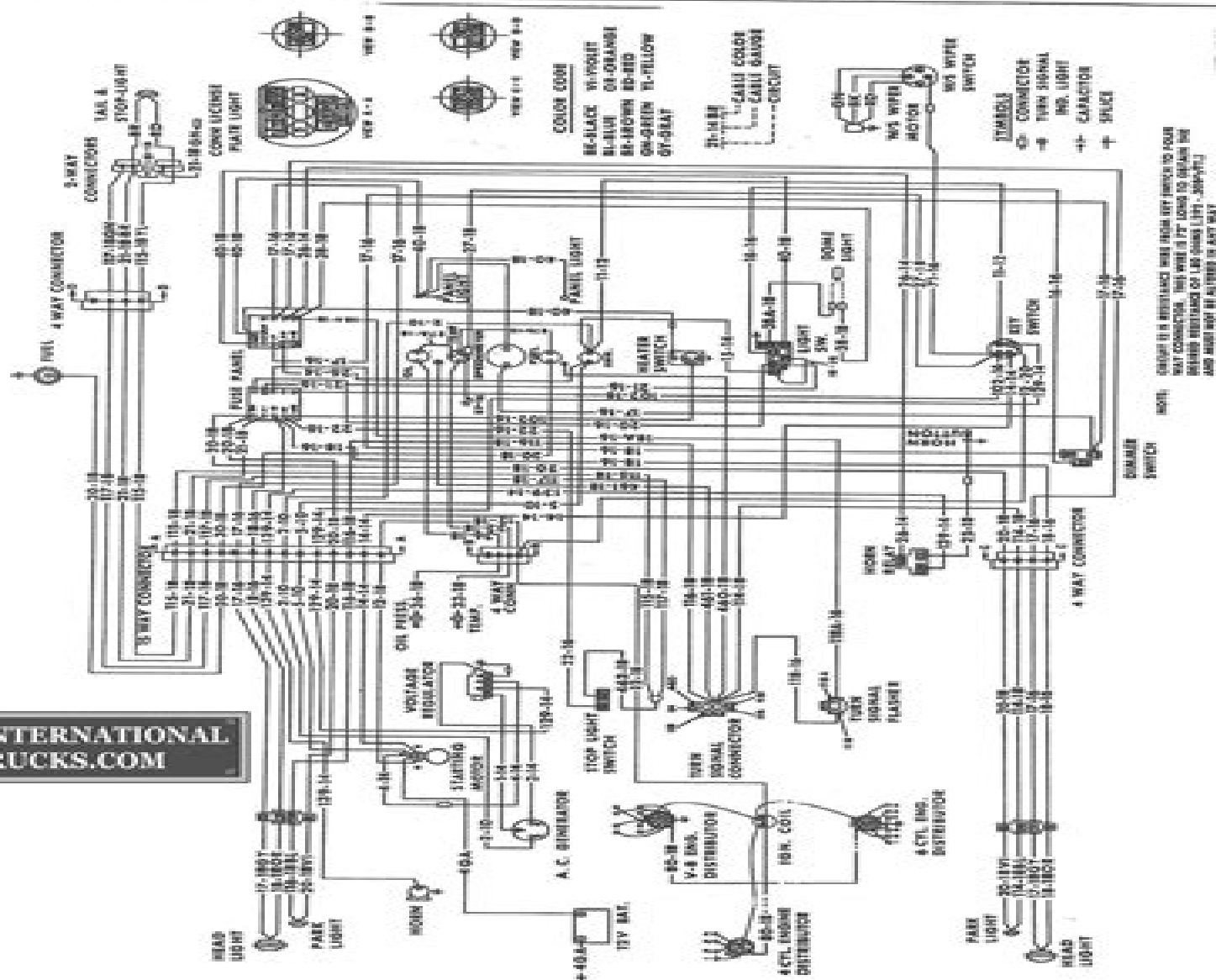
Circuit Diagram C and D-900 Through C and D-1500 With Gasoline Engine
