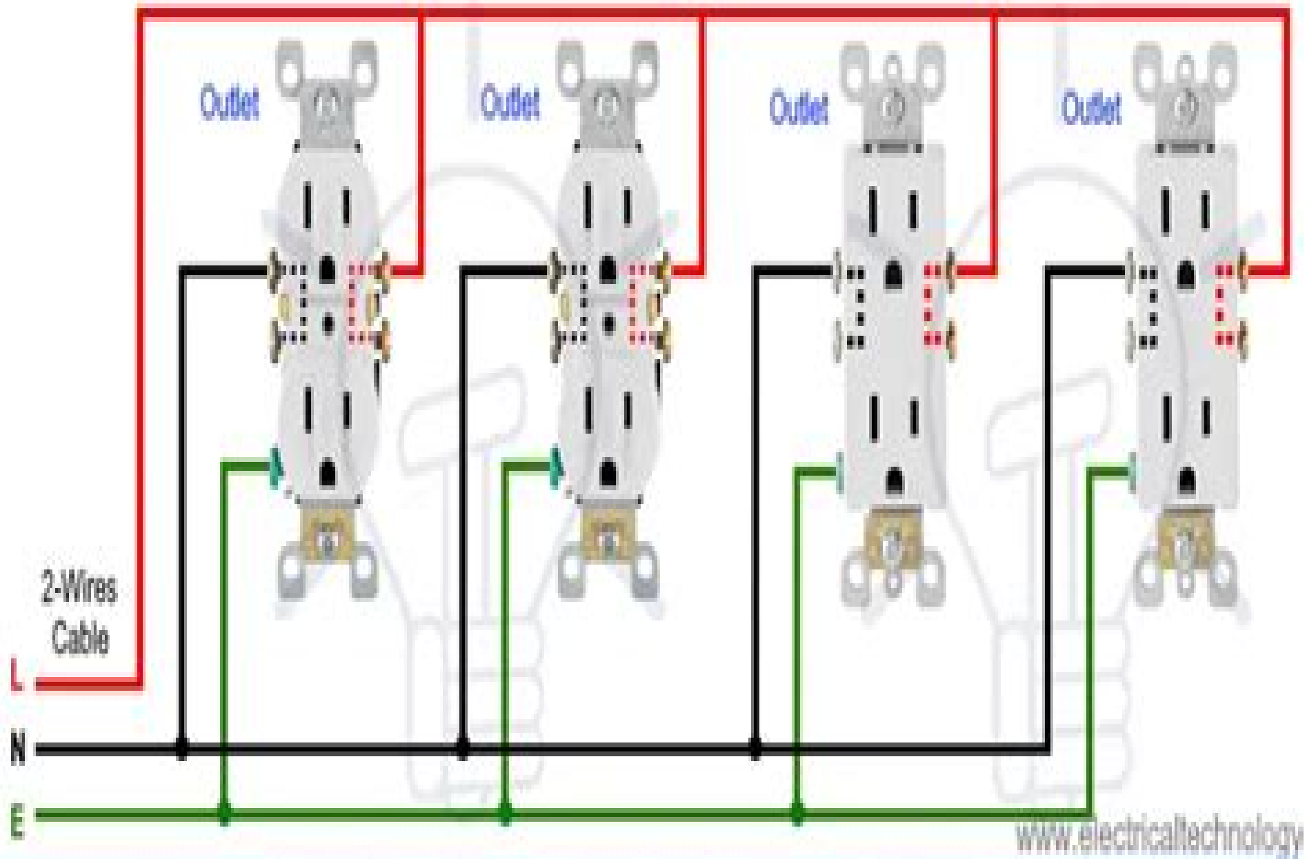
Wiring Multiple Outlets in Parallel
