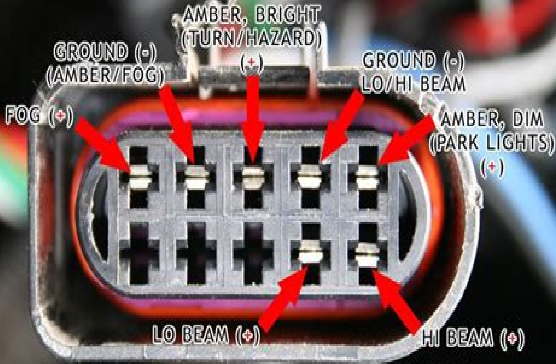
U.S. / NORTH AMERICAN SPEC VOLKSWAGEN MKIV GOLF/JETTA HEADLIGHT HARNESS (CAR SIDE)
