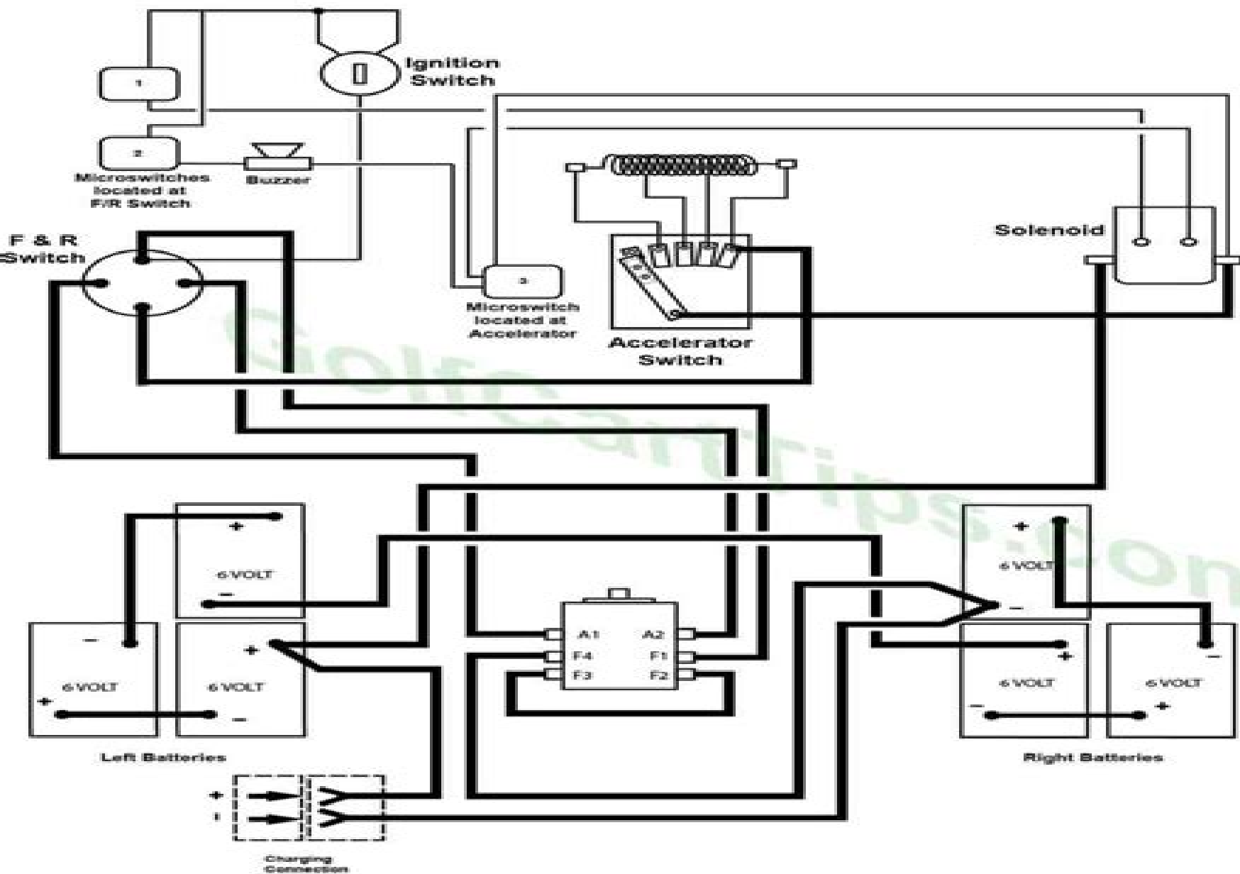
E-Z-GO 400H Wiring Diagram
