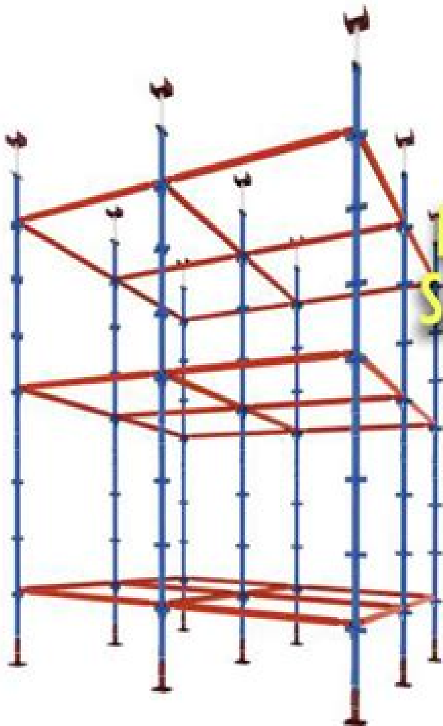
Hammer Scaffolds Horizontal Parts
