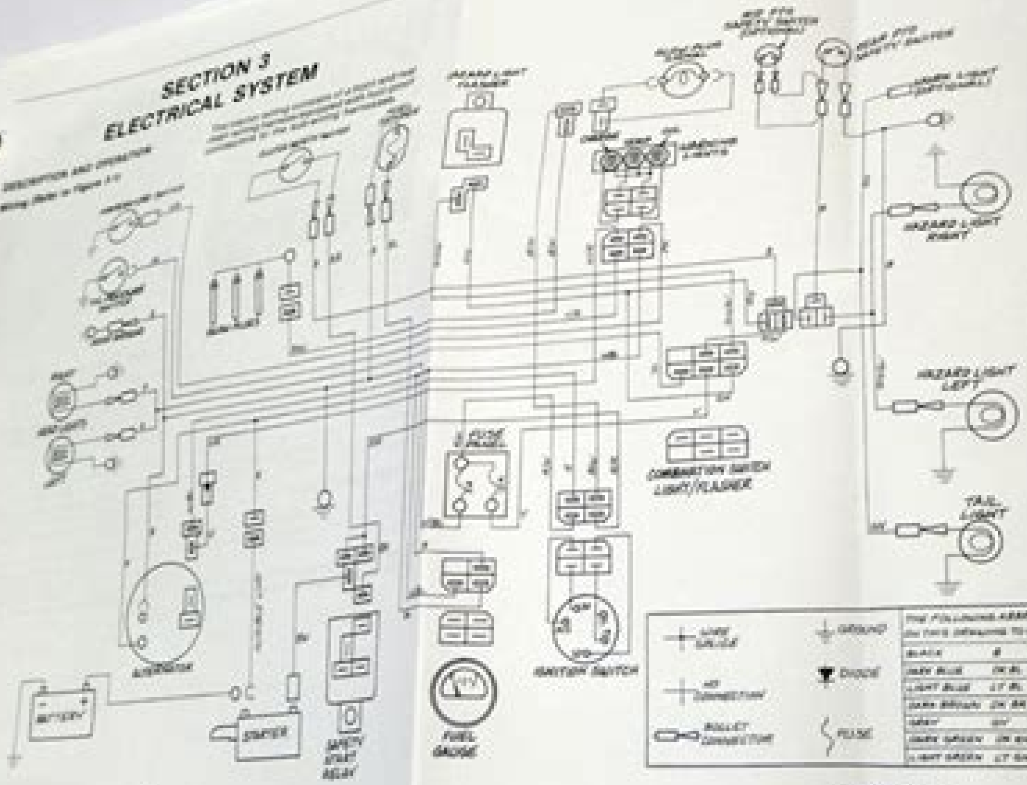
Electrical Diagram
