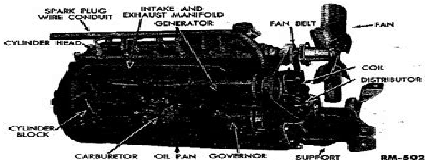
Fig. 2—Right \frac{3}{4} Front View of Engine
