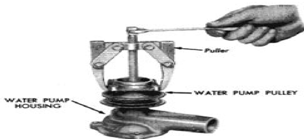
Fig. 33—Removing Water Pump Pulley
