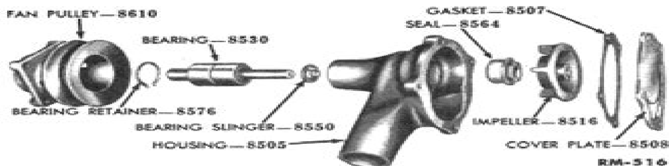
Fig. 34—Water Pump, Disassembled
