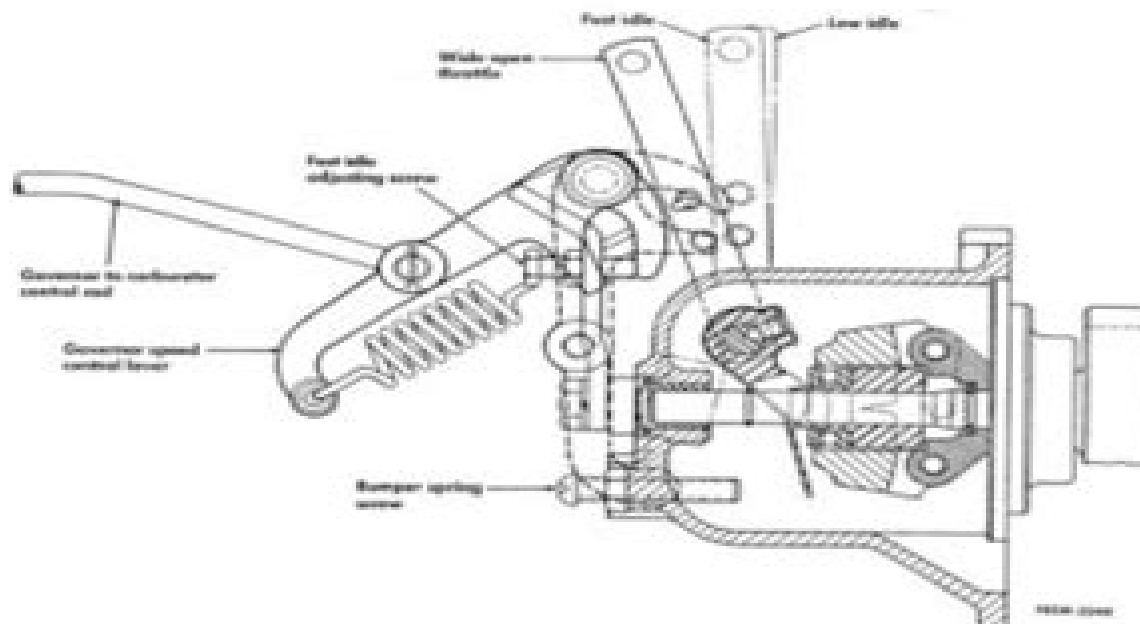
Fig. 1-M. Cross section of engine governor (new style).
