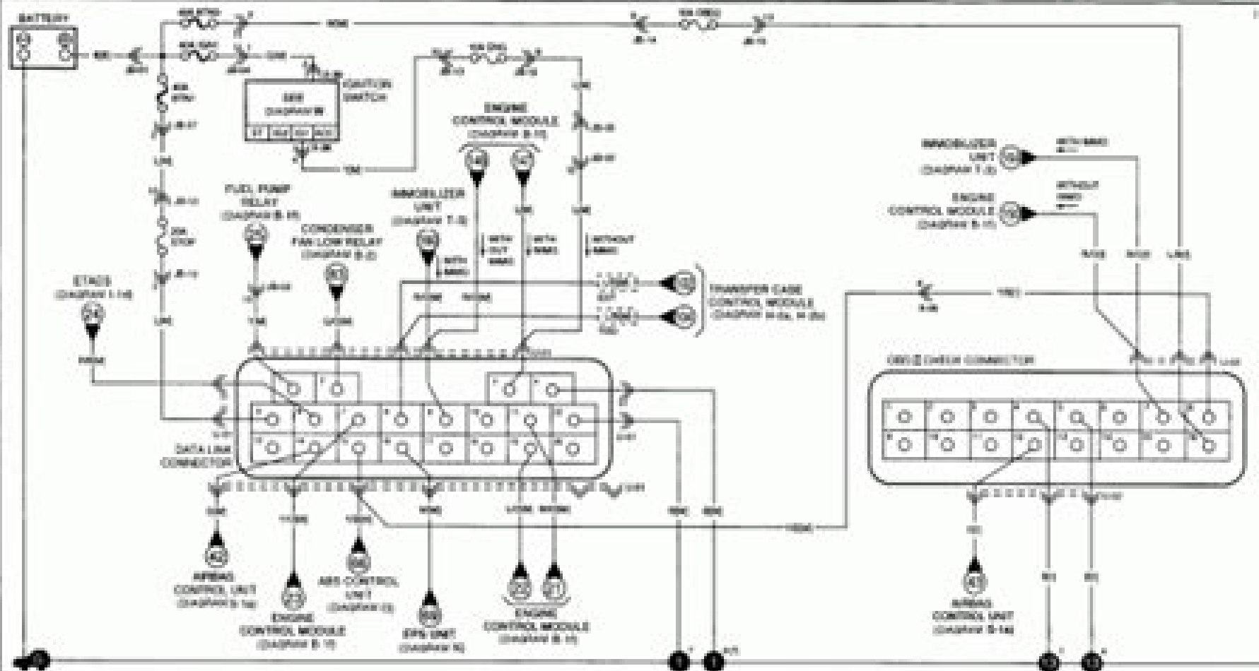
U-101 DATA LINK CONNECTOR (W-1)
