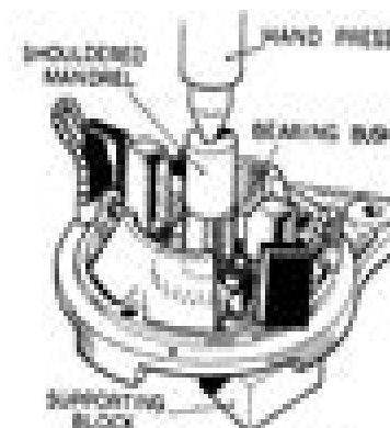
Fig. 20. Method of fitting the inner bearing bush.
