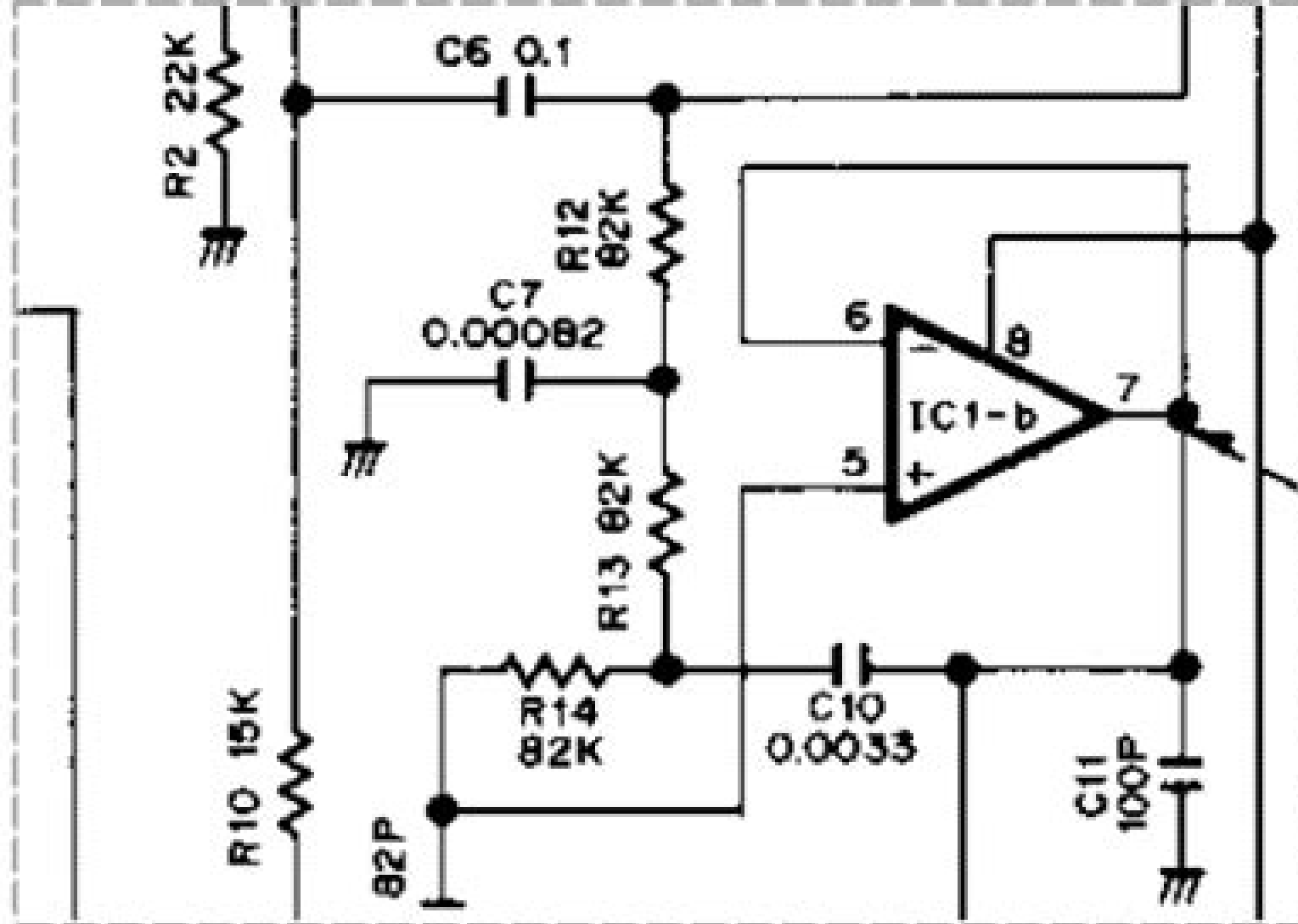
Preview: ICOM IC-229A /E /H schematic diagram
