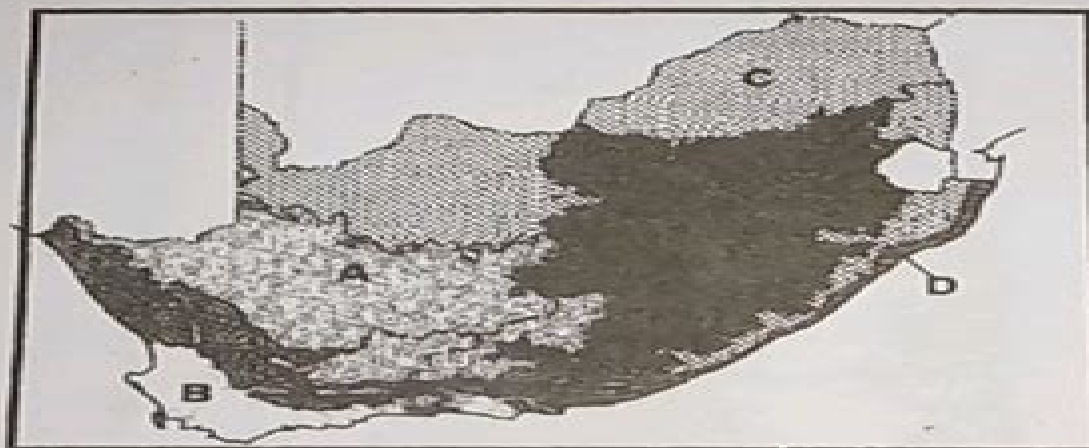
Biomes of South Africa
