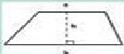
Area of Trapezoid
