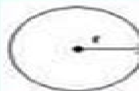
Circumference of a Circle and Area of a Circular Region
