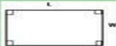
Area and Perimeter of Rectangle
