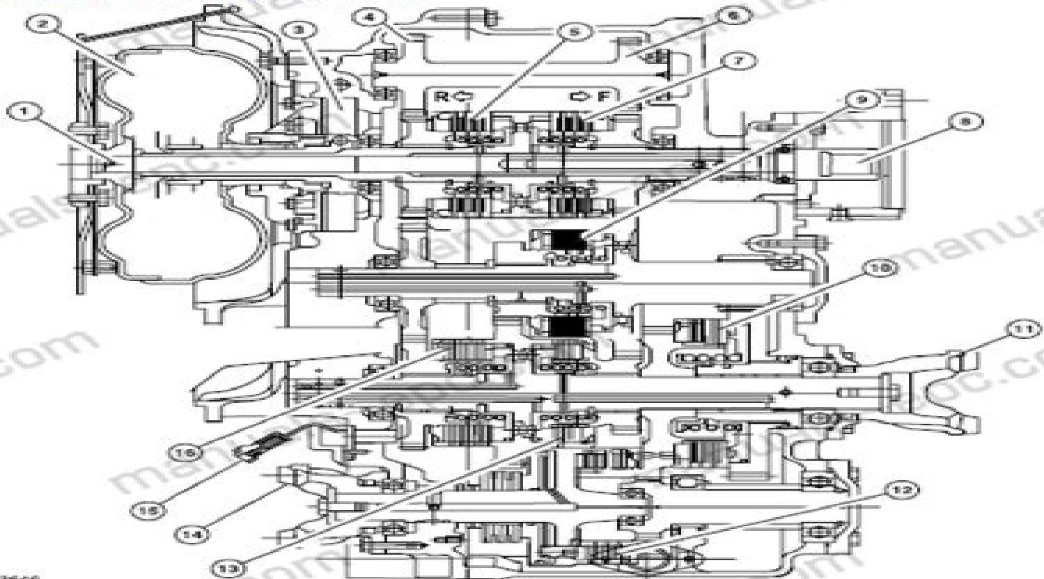
Schematic View Powershift Transmission
