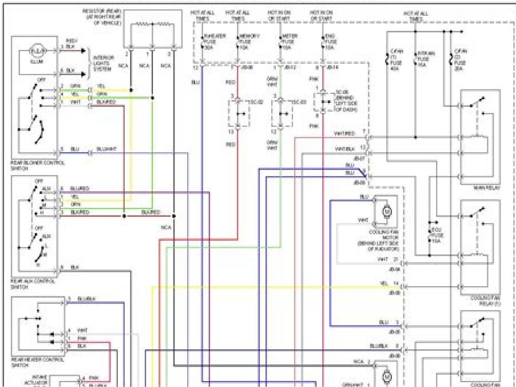
2002 Kia Sedona EX-Fig. 2: Manual A/C Circuit (2 of 2)
