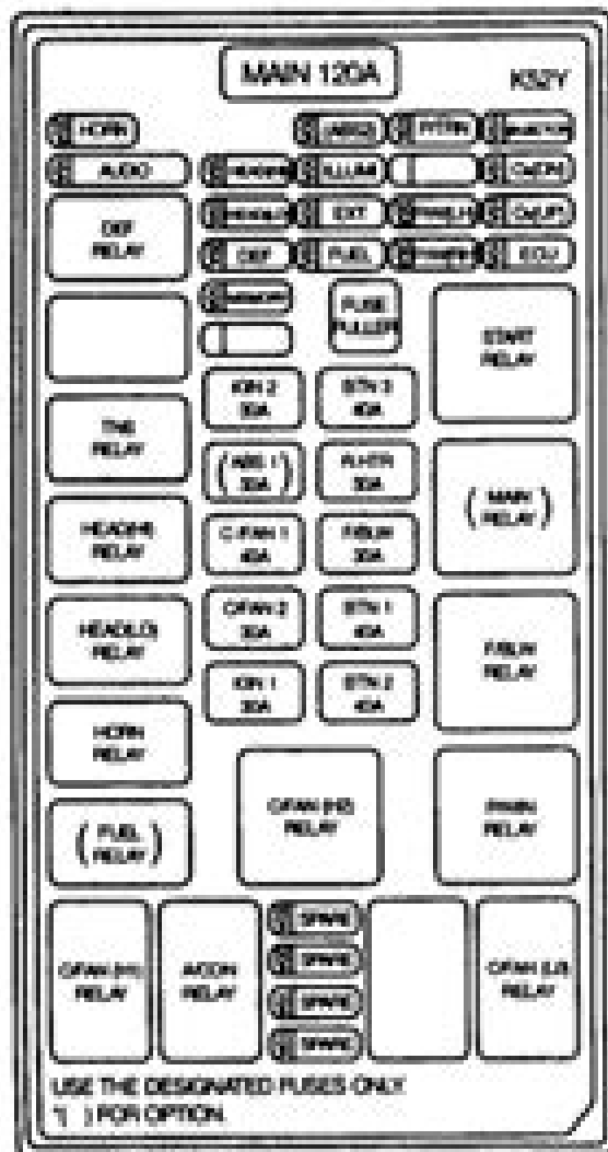
Fig 4: Locating & Identifying Components On Engine Compartment Fuse/Relay Box
