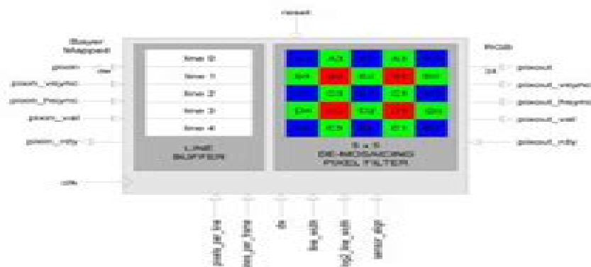
Figure 1: Bayer-to-RGB converter architecture
