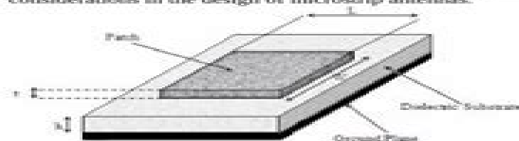
Fig.1. Basic Structure of a Microstrip Patch Antenna
