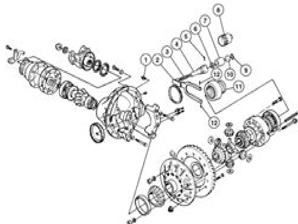
Differential lock assembly
