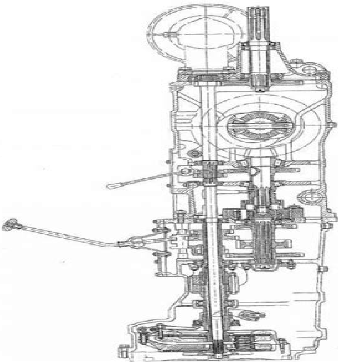
Fig. 11. - Transmission longitudinal section.
