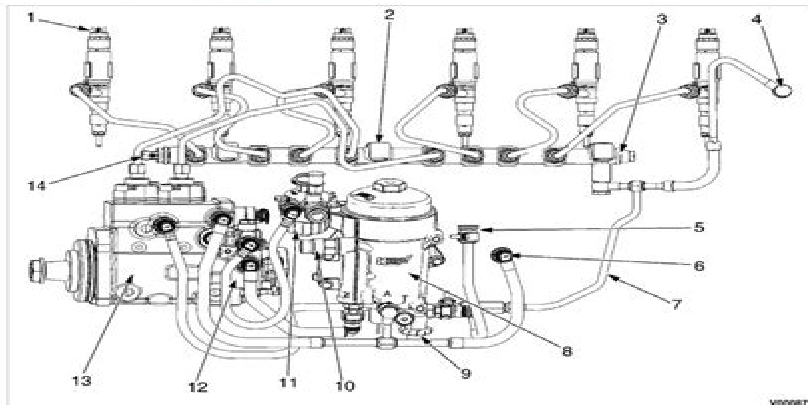
Figure 16 Fuel system
