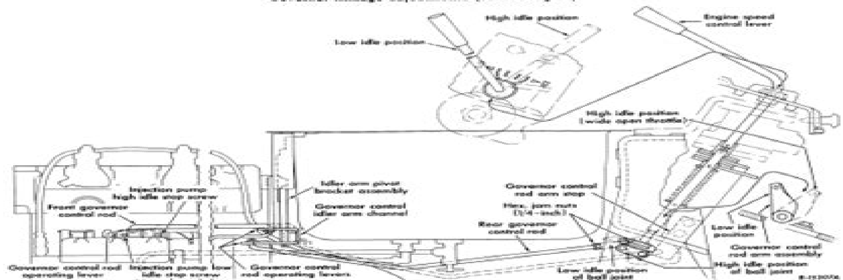
Illustr. 51A Governor linkage adjustments (diesel engine).
