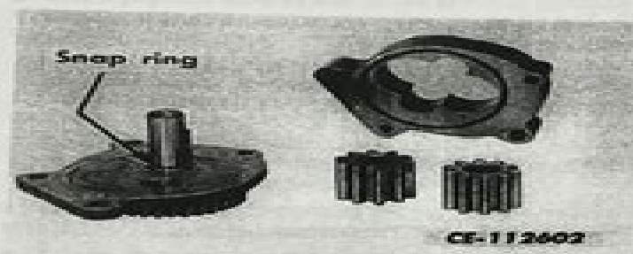
Fig. 12. Removing or Installing Old Style Drive Shaft
