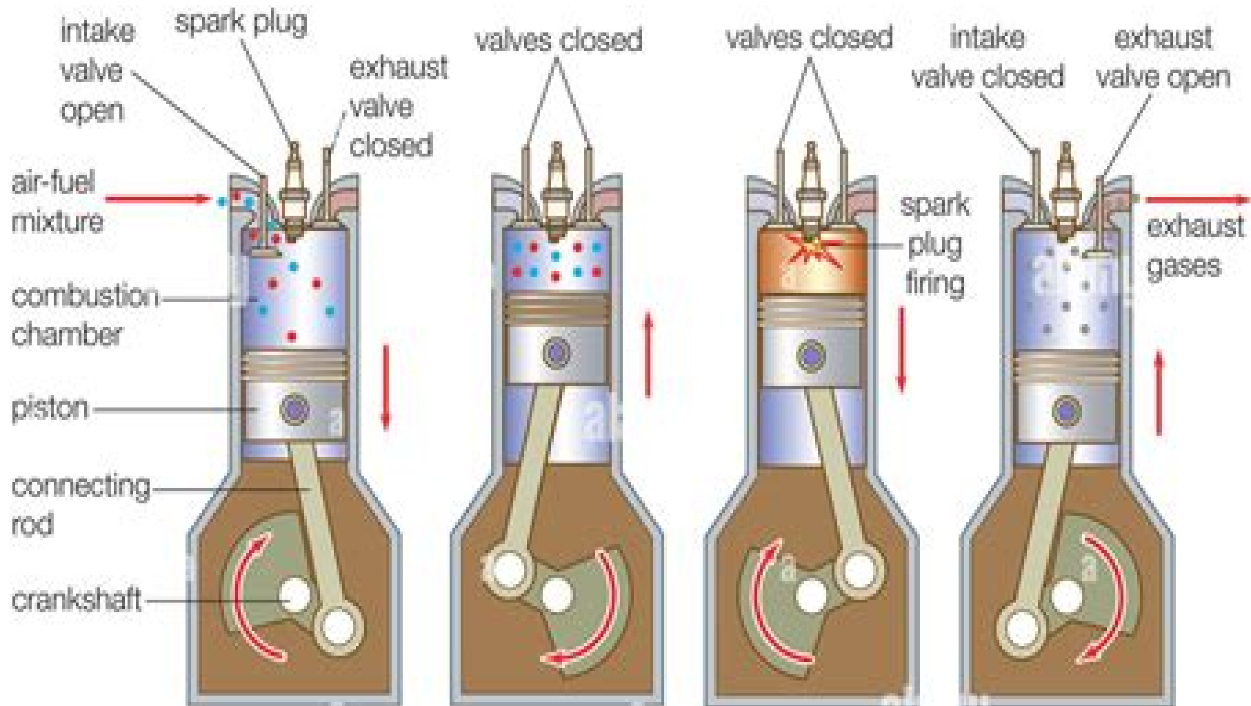
intake Air-fuel mixture is drawn in.
