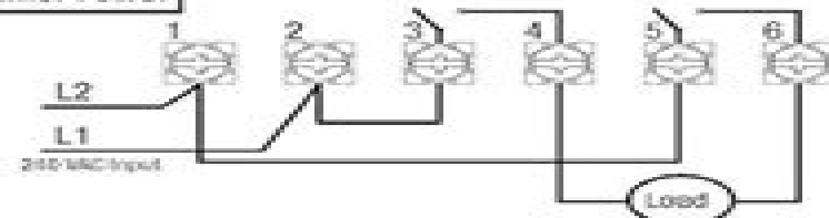
Timer Power
