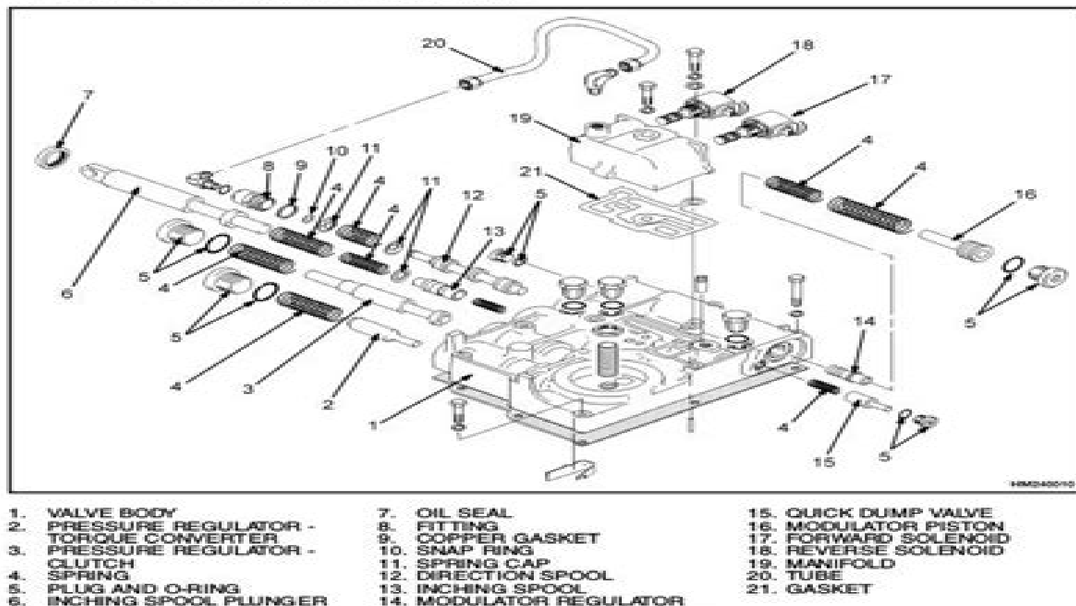
Figure 12. Control Valve - Later Model S3.50-5.50XL (S70-120XL) Trucks and S3.50-5.50XM (S70-120XM) Trucks
