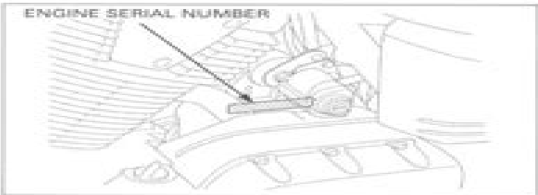
(2) The engine serial number is stamped on the right side of the upper crankcase.
