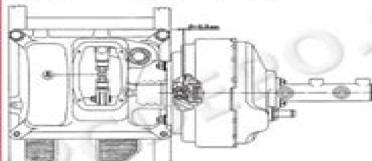
Fig. 6 - CLEARANCE OF BRAKE BOOSTER PUSH ROD. A - Adjusting the rod.
