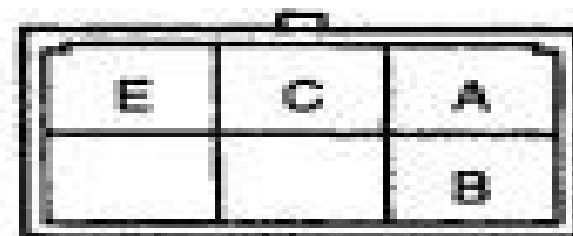
PART SIDE CONNECTOR (VIEW FROM TERMINAL SIDE)
