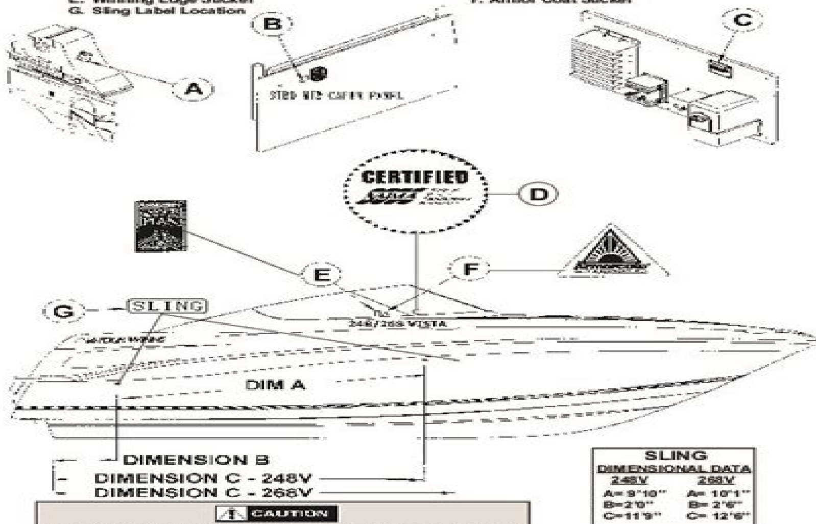
Figure 2: 248/268V ADDITIONAL LABEL/STICKER LOCATIONS
