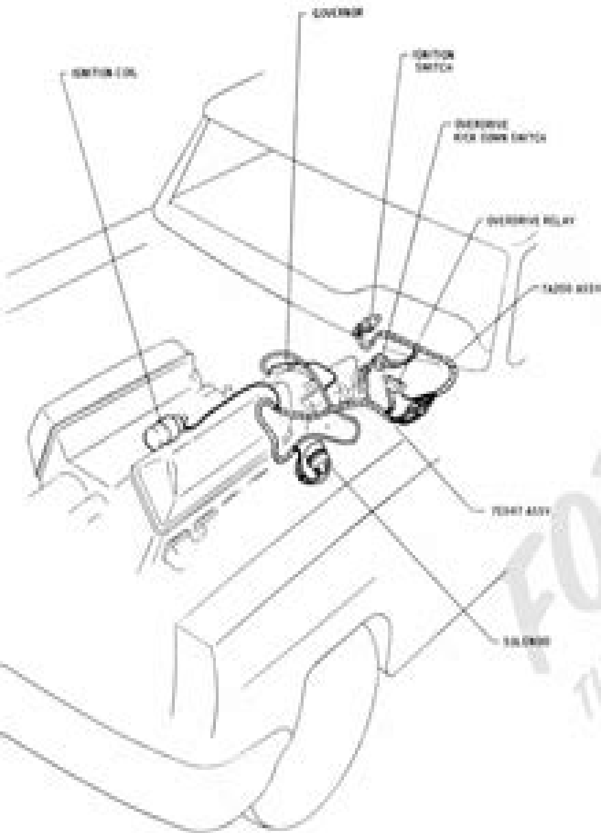
1967 FORD OVERDRIVE
