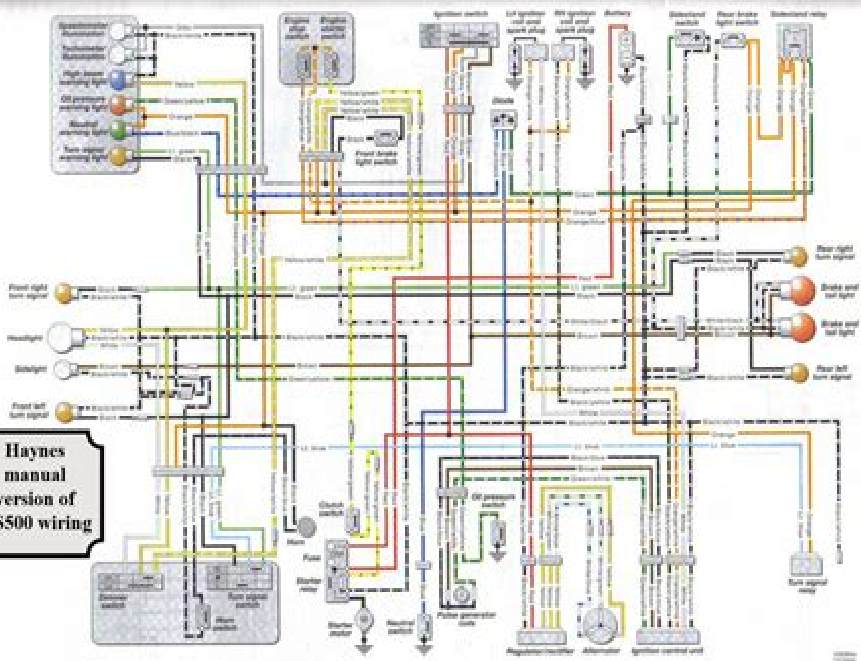
Wiring diagram - US GS500 EL, M, N, P, R, S and T models
