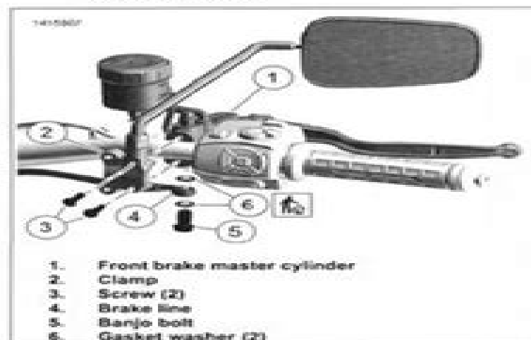
Figure 3-28. Front Brake Master Cylinder Mount
