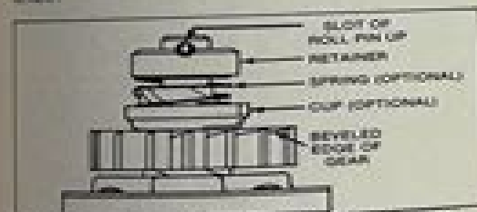
Fig. 88 — Assembling Starter Motor Drive
