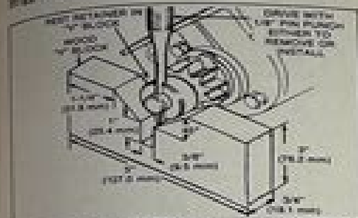
Fig. 87 — Disassembling Starter Motor Drive
