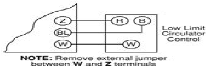
Figure 7. Alternate Connections for using Separate Low Limit-Circulator Control on Boiler with Tankless Domestic Coil
