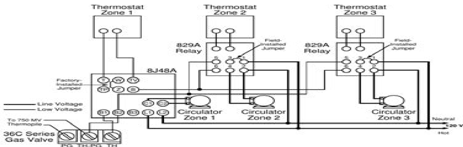
Figure 9. 8J48A - Millivolt Systems Zoned with Circulators
