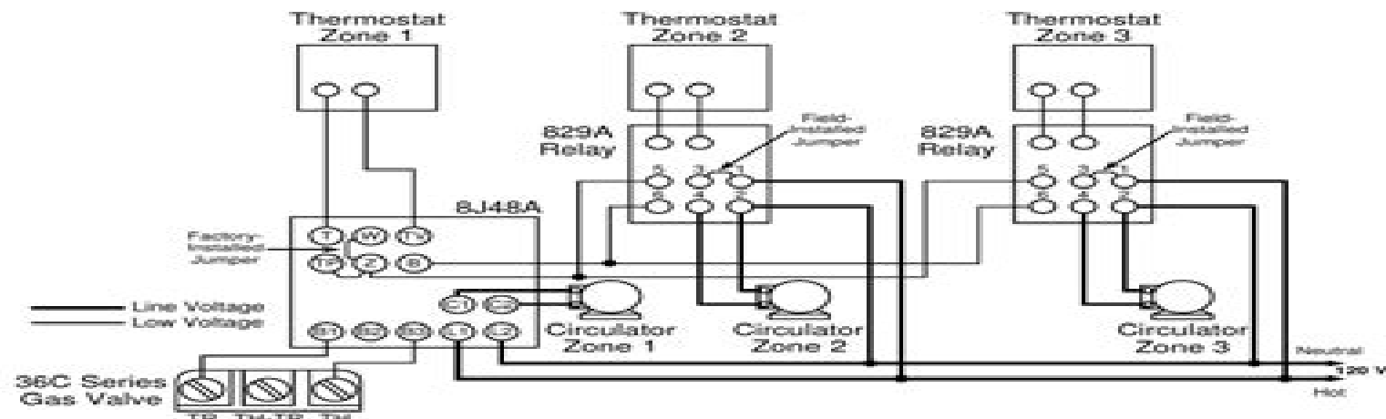
Figure 8. 8J48A - 24 Volt Systems Zoned with Circulators
