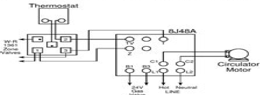
Figure 6. Typical Connections for Zoning with 2-Wire Zone Valves
