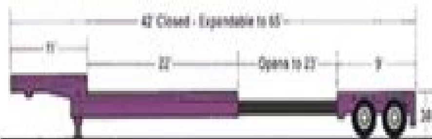
EXTENDIBLE (STRETCH) DROPDECK
