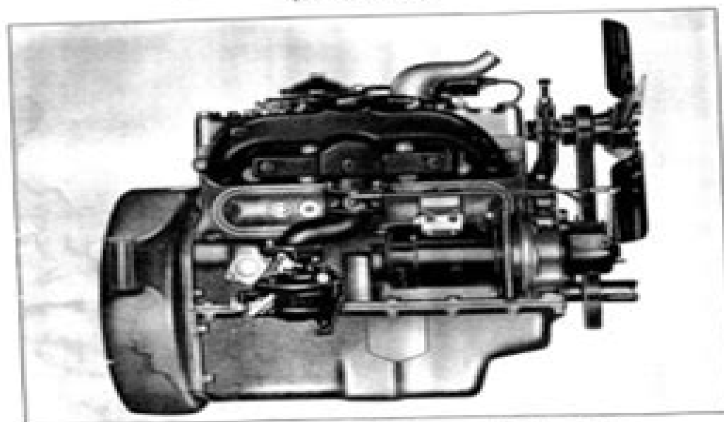
JX 4-2 Series Camshaft, Manifold, Governor and Fuel Pump Side (Right Hand Side)
