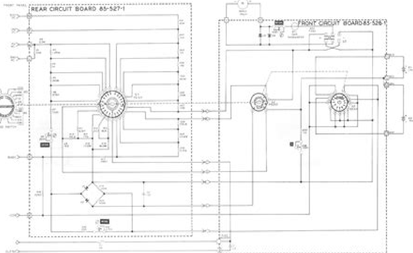
SCHEMATIC OF THE HEATHKIT® VOLT-OHM-MILLIAMMETER MODEL IM-105
