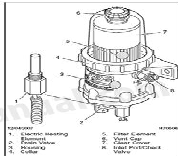
Fig. 1, Fuel Pro 382 With Electric Heating Element
