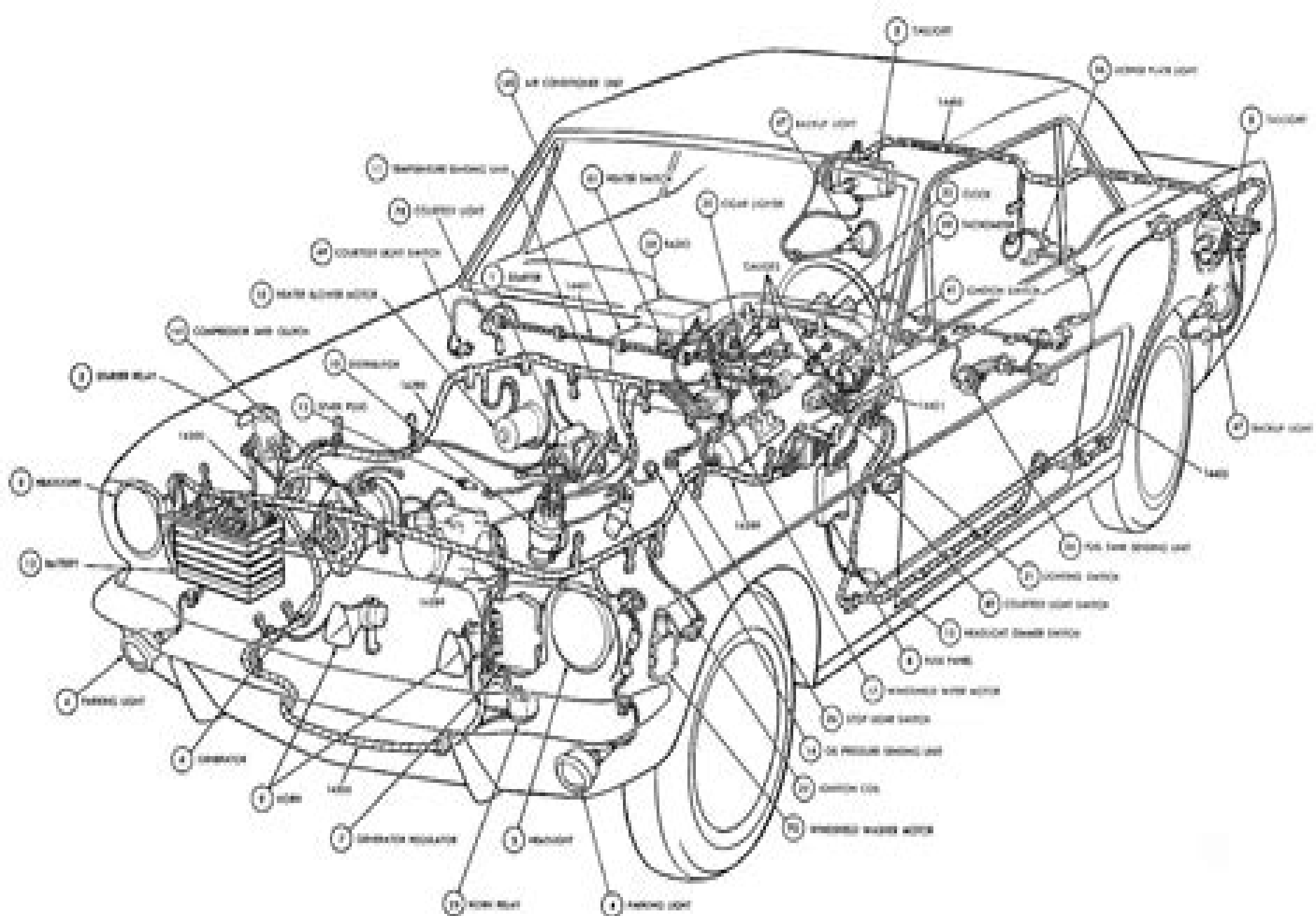
1964 MUSTANG MASTER WIRING LOCATOR
