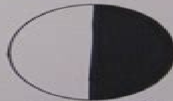
Third Quarter
