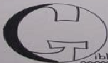
Waxing Gibbous
