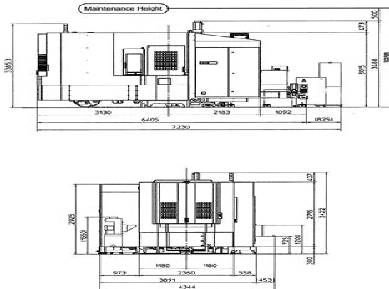
Figure 2.9 Front and Side View of Machine: a82 (Tool Magazine A40 and Left Discharge Lift-Up Conveyor Spec.)
