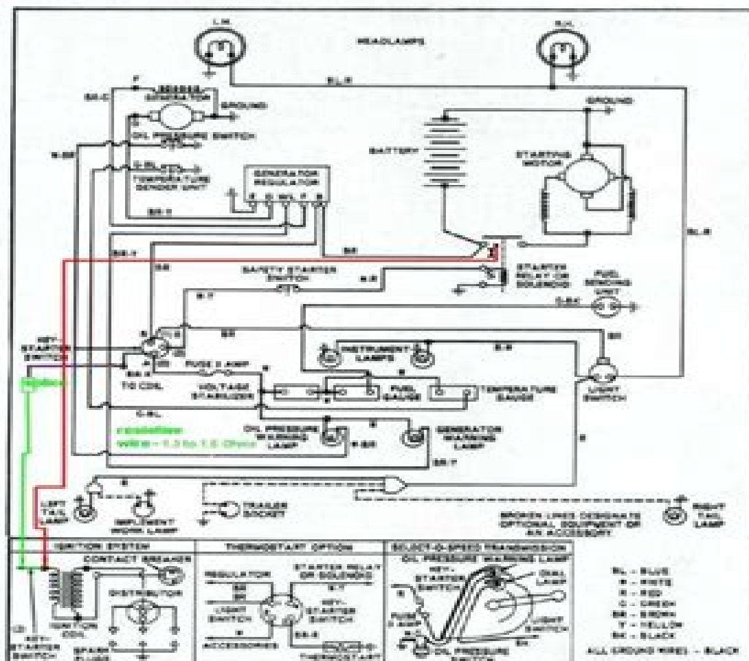
Fig. 140—Wiring diagram for all models with "C" prefix to tractor serial number. Refer to page 2 of this manual for serial number location. For tractors with "A" or "B" prefix to tractor serial number, refer to Fig. 161.
