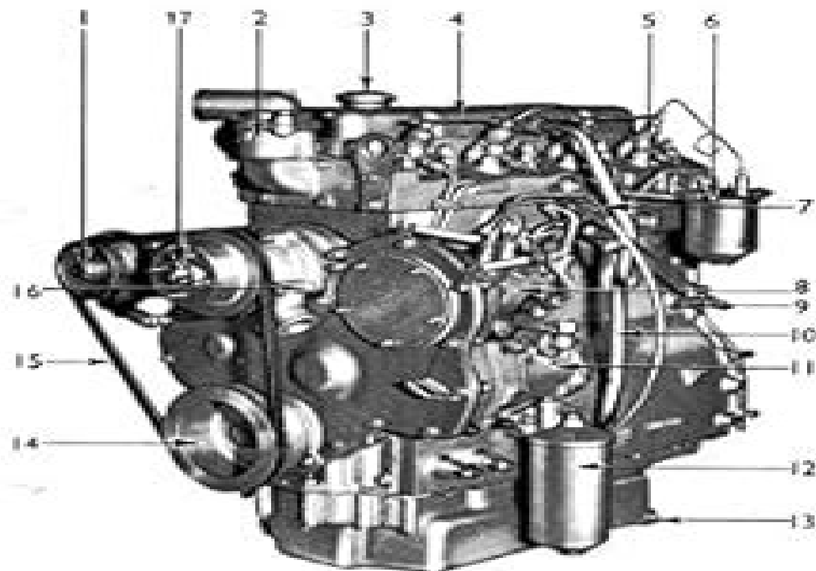
VIEW OF FUEL PUMP SIDE OF ENGINE (4.200 Phase 1 Black)
