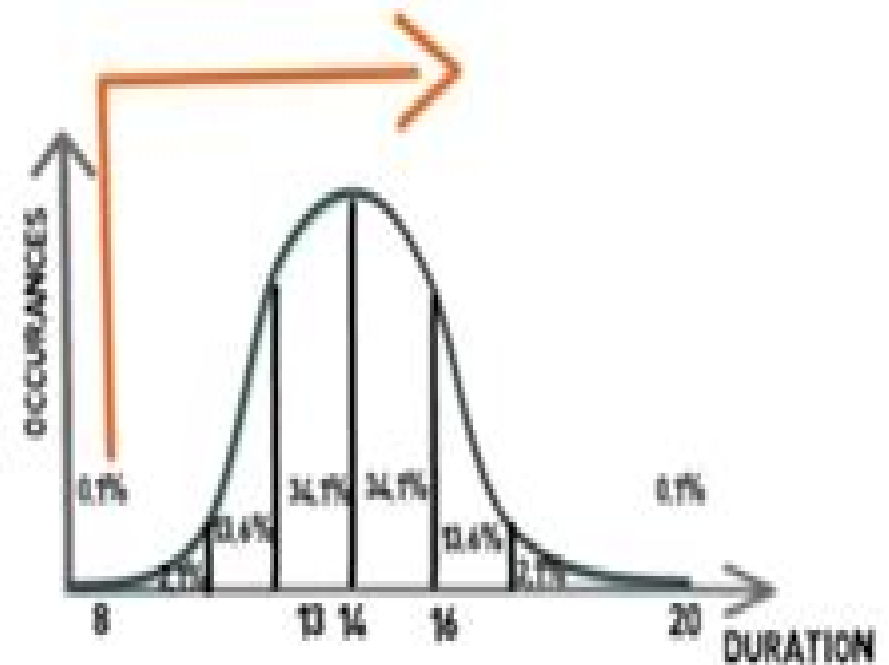
PROBABILISTIC DISTRIBUTION
