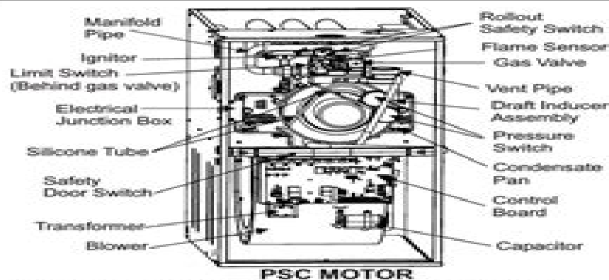
FIGURE 5: Component Location - 97% Modulating PSC Models
