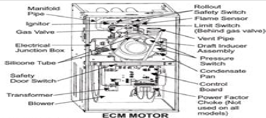
FIGURE 6: Component Location - 97% Modulating ECM Models
